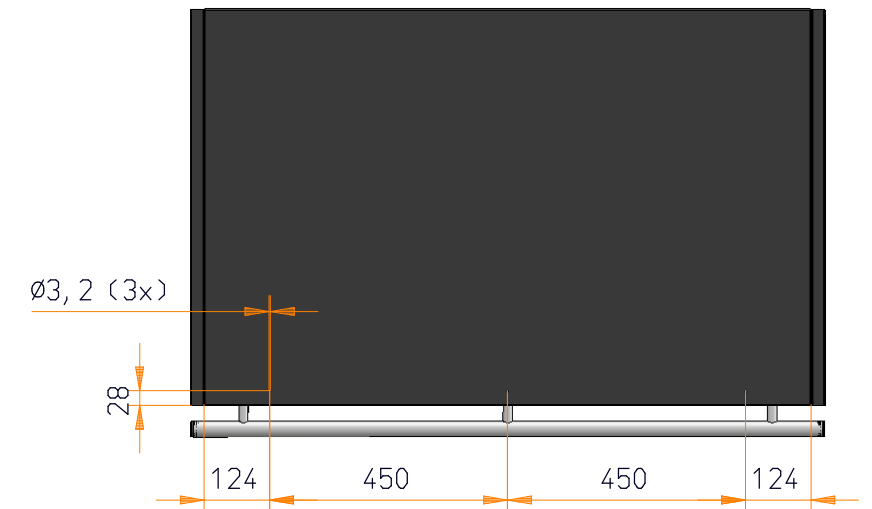
Panel dimensions
