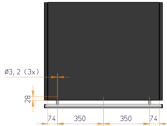
Panel dimensions
