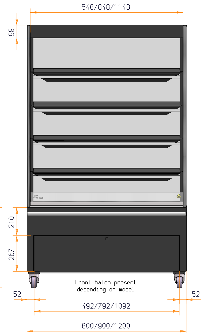
Panel dimensions
